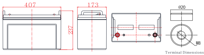
Terminal Dimensions
