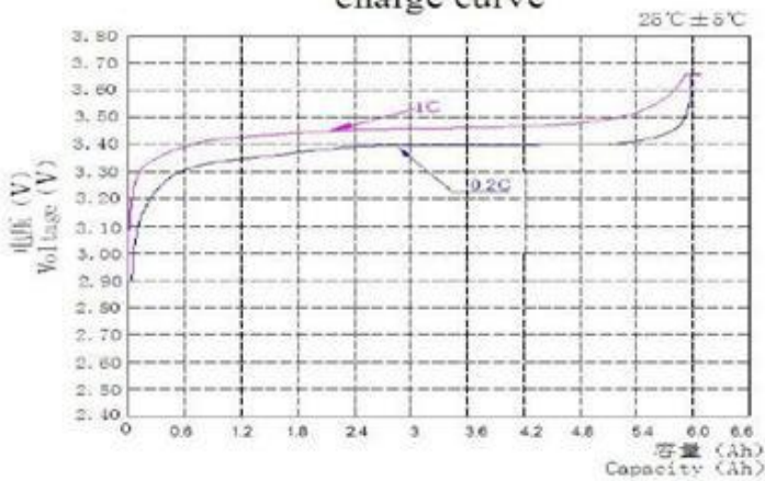
充电曲线图 charge curve
